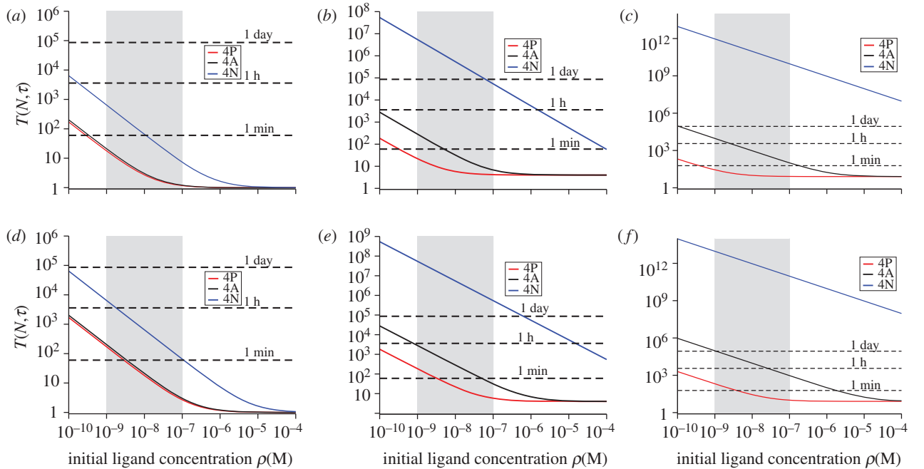
Figure 6. Mean time to signal initiation (MTSI) for a T cell according to the stochastic criterion. MTSI, T(N, \tau) , for double positive thymocytes (DP), T1 TCRs at 37 degrees. Different panels stand for different pairs of values (N, \tau) : (a) for (10, 1) , (b) for (10, 4) , (c) for (10, 8) , (d) for (100, 1) , (e) for (100, 4) and (f) for (100, 8) . Time units are seconds. The physiologically relevant range of initial ligand concentration is shaded grey, and the dotted lines correspond to a time scale of 1 min, 1 h and 1 day, respectively.
