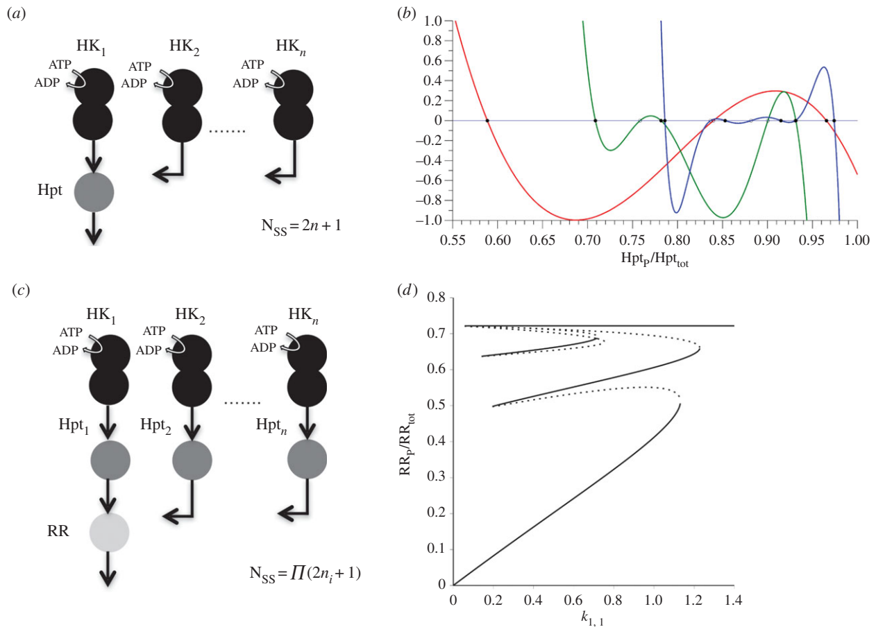
Figure 3. Cartoon representation of sharing of downstream components at the level of Hpt ( a ) or RR ( c ). ( b ) Plot of the polynomial function (see the electronic supplementary material, SI-1) characterizing the steady-state level of the phosphorylated Hpt for the system shown in ( a ) for a specific set of parameter values (see the electronic supplementary material, table S1). Both the polynomial and the variable are scaled to the shown window. The polynomial is plotted in red, green and blue for one, two and three HKs, respectively. Each crossing of the polynomial with the x -axis is a steady state of phosphorylated Hpt. Stable and unstable steady states are shown as filled and open circles, respectively. ( d ) Bifurcation plot for a system with two hybrid HKs, each with separate Hpts that share the same RR (as shown in ( c ), for n = 2 ). We assume that the auto-phosphorylation rate constants for HK 1 and HK 2 (when the REC site is unphosphorylated) are the same and determined by the same signal (i.e. k_{1,1} = k_{2,1} ). The bifurcation plot shows the fraction of phosphorylated RR at steady state for a given input level ( k_{1,1} = k_{2,1} ). The parameter values are chosen such that the system displays nine distinct steady states (see the electronic supplementary material, table S1). The solid and dotted lines indicate stable and unstable steady states, respectively.
